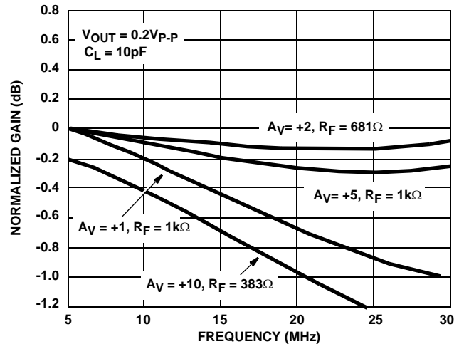
FIGURE 26. NON-INVERTING GAIN FLATNESS vs FREQUENCY
